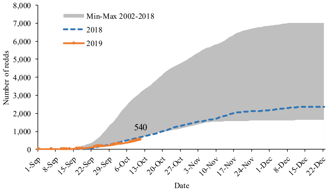
Figure 2. Cumulative redd counts in Reaches 1–10 (Reach 8 excluded) of the mainstem Trinity River in 2019 as of October 11 compared to 2018 and the range of counts from 2002 to 2018.
