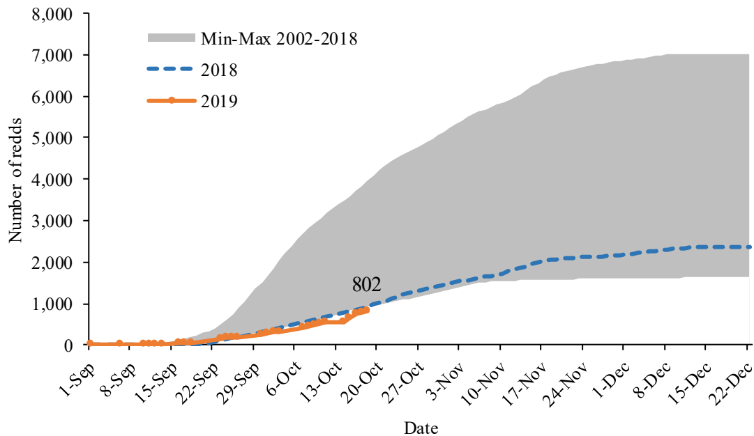
Figure 2. Cumulative redd counts in Reaches 1–10 (Reach 8 excluded) of the mainstem Trinity River in 2019 as of October 18 compared to 2018 and the range of counts from 2002 to 2018.
