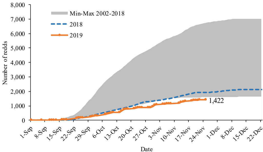
Figure 2. Cumulative redd counts in Reaches 1–10 (Reach 8 excluded) of the mainstem Trinity River in 2019 as of November 29 compared to 2018 and the range of counts from 2002 to 2018.
