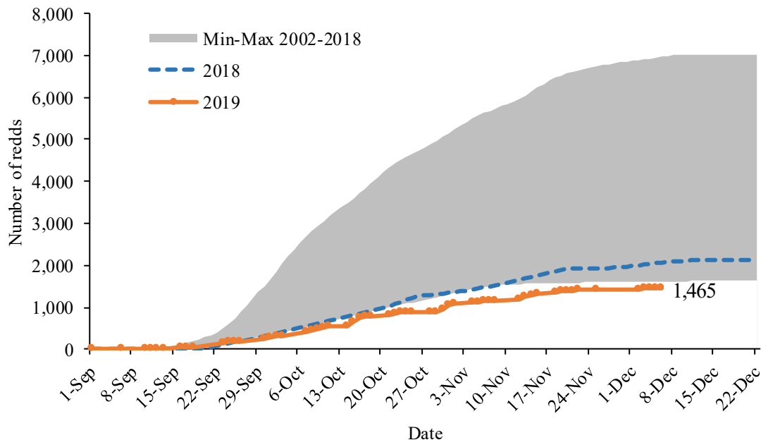
Figure 2. Cumulative redd counts in Reaches 1–10 (Reach 8 excluded) of the mainstem Trinity River in 2019 as of December 6 compared to 2018 and the range of counts from 2002 to 2018.
